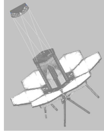
Figure 2. High fidelity finite element model.
